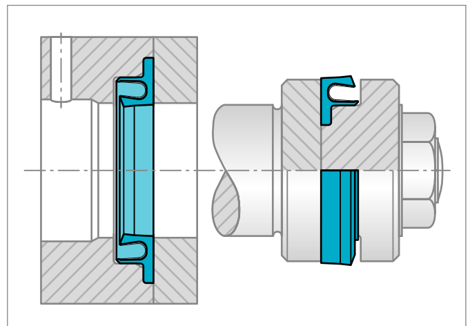
Figure 154: Installation of Variseal®
