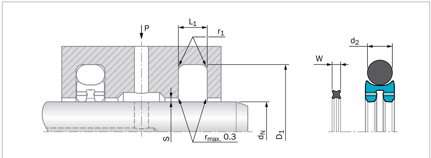
Figure 131 Installation Drawing
