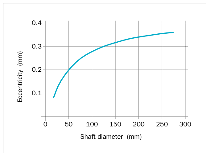
Figure 57: Permissible eccentricity
