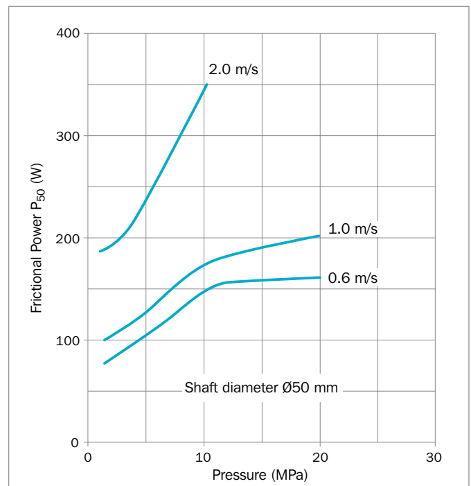
Figure 130 Frictional power for Turcon® Roto Glyd Ring® V in Turcon® M15
