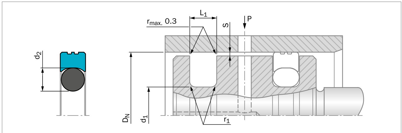
Figure 121: Installation Drawing
