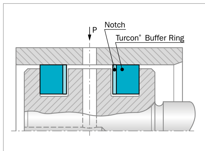
Figure 170: Right installation of Turcon® Buffer Ring
