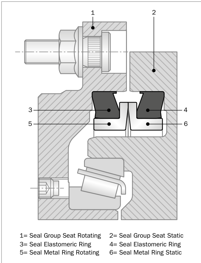
Figure 174: Mechanical Face Seals, Type DF
