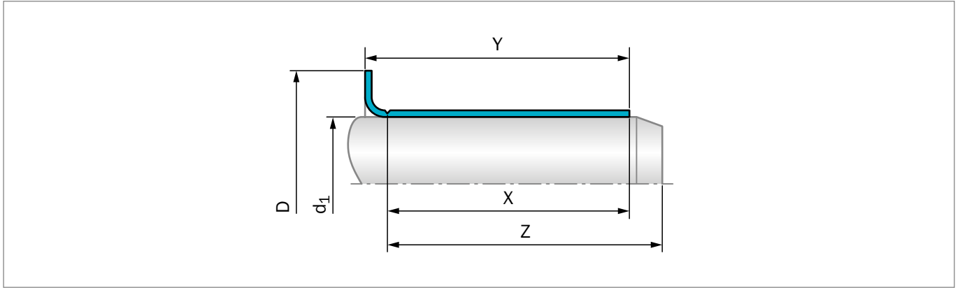
Figure 69: Installation Drawing
