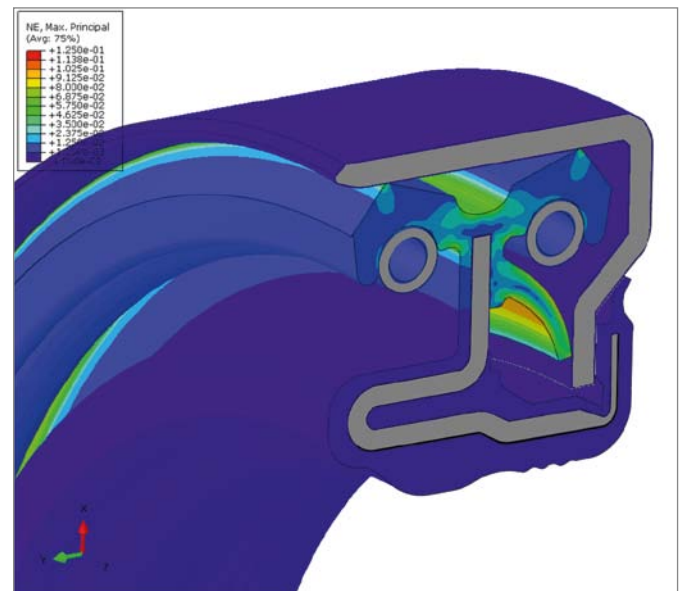
Figure 49: Friction optimization through FEA
