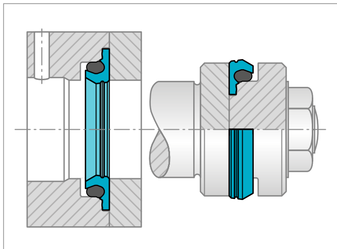
Figure 155: Installation of rod Turcon® Roto Variseal® and Roto VL Seal® F in split groove
