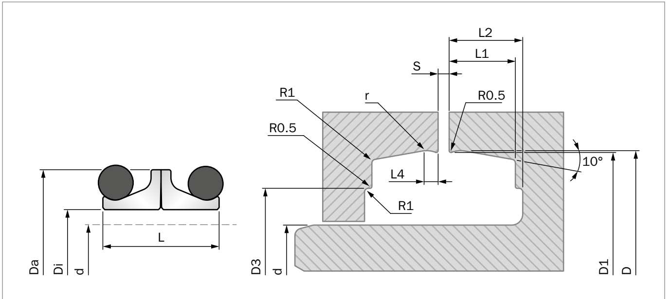
Figure 185: Installation Drawing
