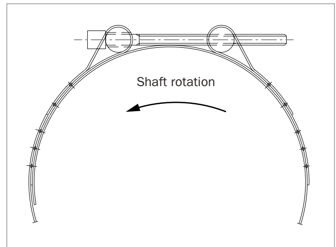
Figure 74: Clamping band RM
