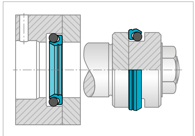
Figure 153: Installation of Roto VL Seal® in split grooves
