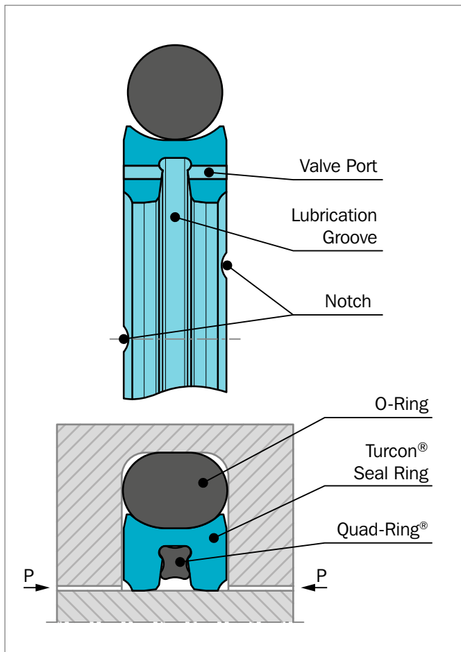
Figure 127 Turcon® Roto Glyd Ring® V with pressure relief
