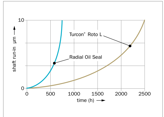
Figure 94: Lifetime of hardware
