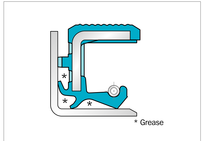
Figure 60: APJ for corrosive applications
