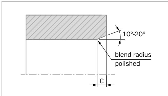
Figure 167: Lead-in chamfer on housing
