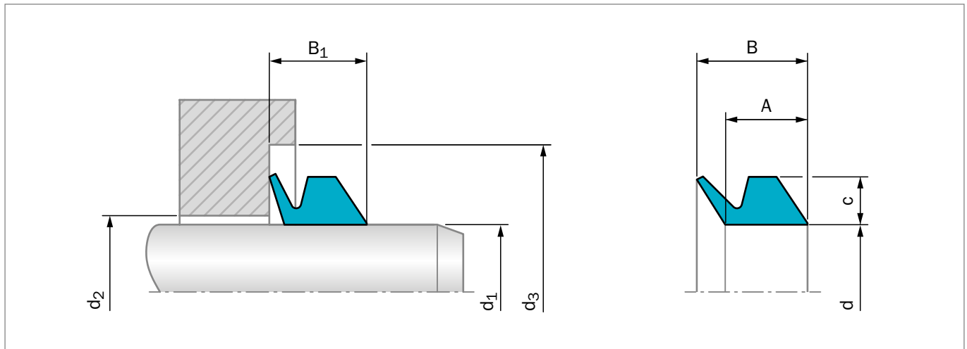
Figure 77: Installation Drawing
