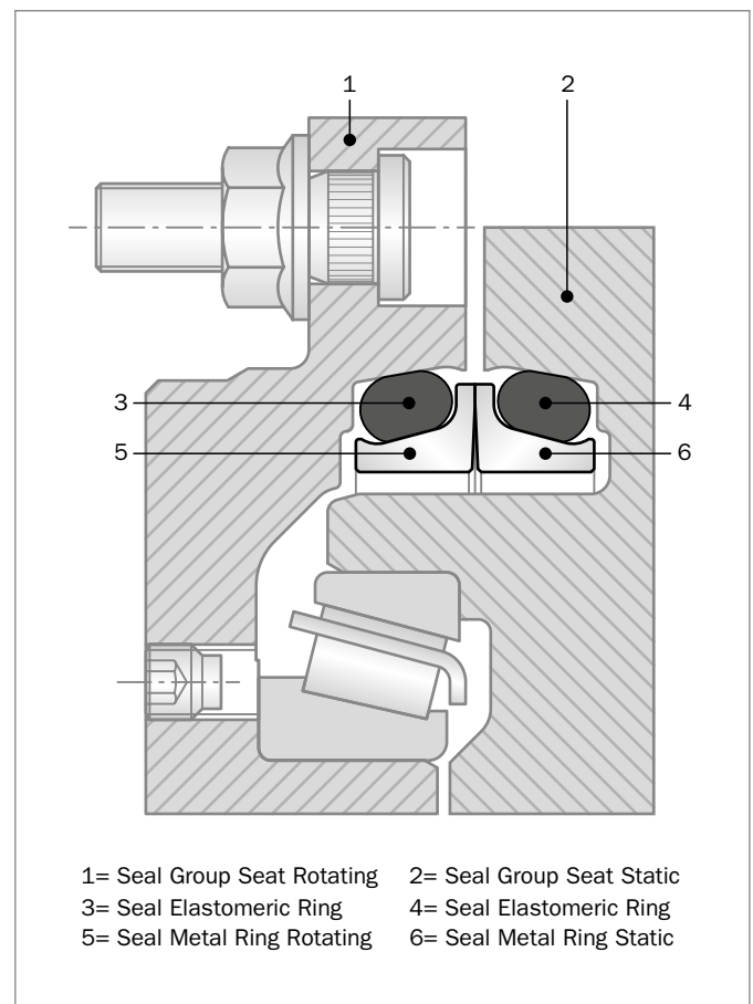
Figure 173: Mechanical Face Seals, Type DO
