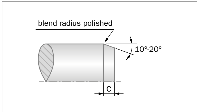
Figure 140 Lead-in chamfer on shaft
