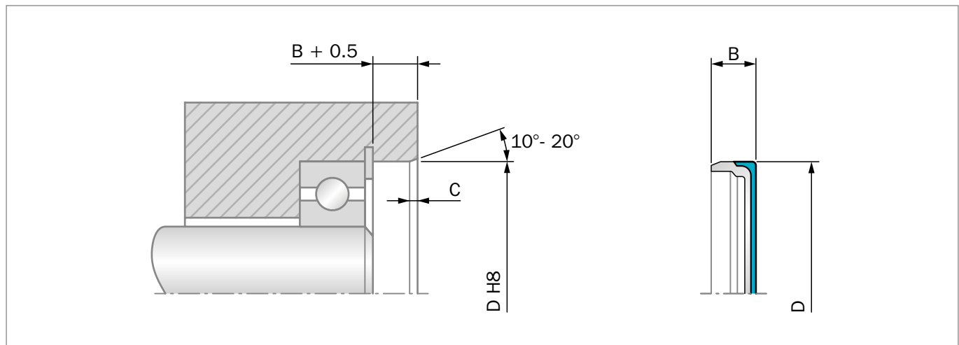
Figure 64: Installation Drawing
