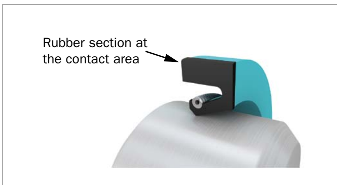
Figure 37: Contact area, split seal
