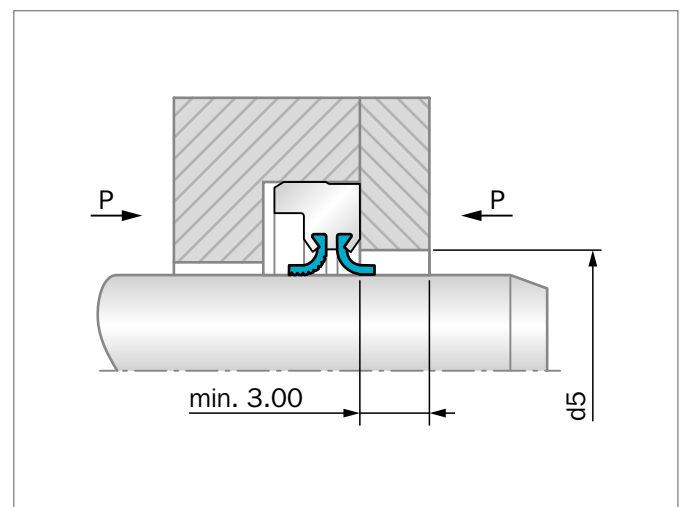
Figure 115: Installation type for fluid separation at pressures up to 0.5 MPa (145 psi)
