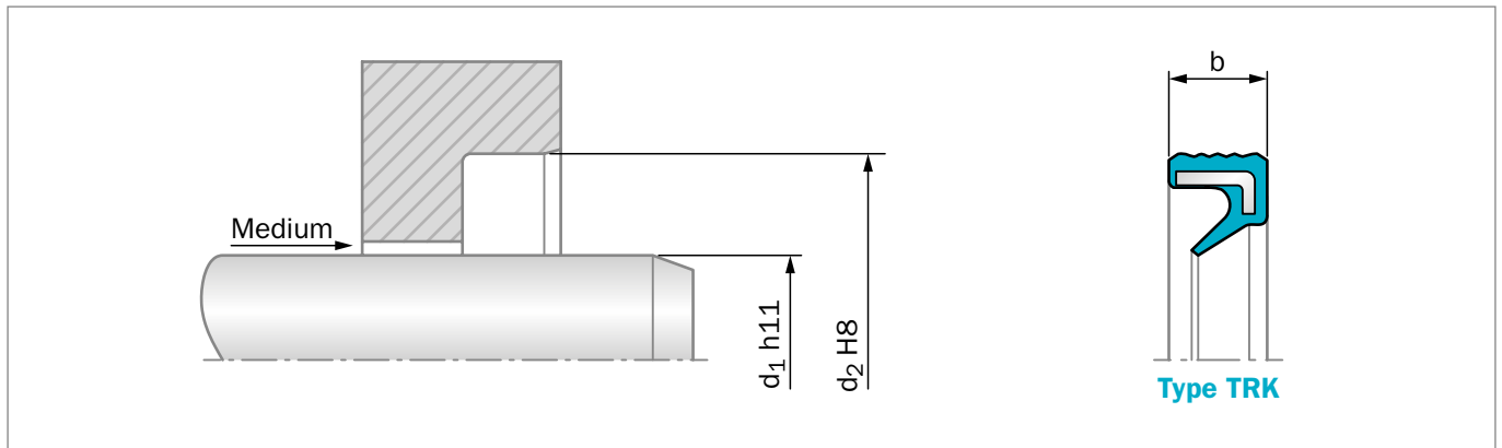
Figure 29: Installation Drawing
