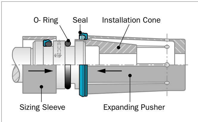
Figure 164: Calibration and installation of bore Turcon® Roto VL Seal® by an Installation Cone and Expanding Pusher
