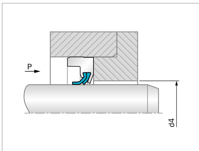
Figure 114: Installation for pressure from 0.5 MPa (73 psi) up to 1 MPa (145 psi)
