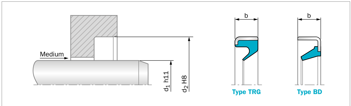
Figure 30: Installation Drawing
