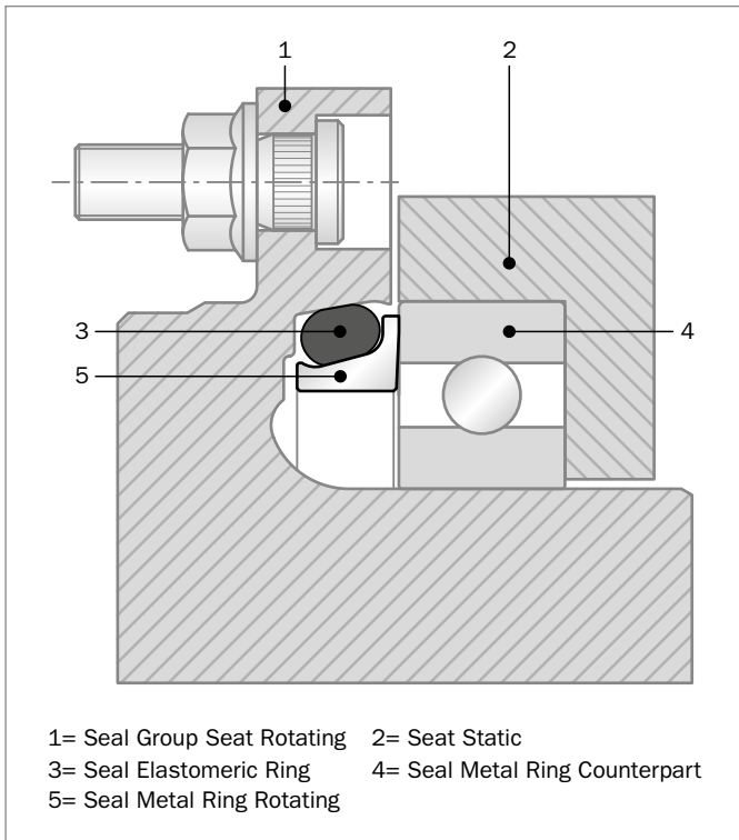
Figure 175: Special Design
