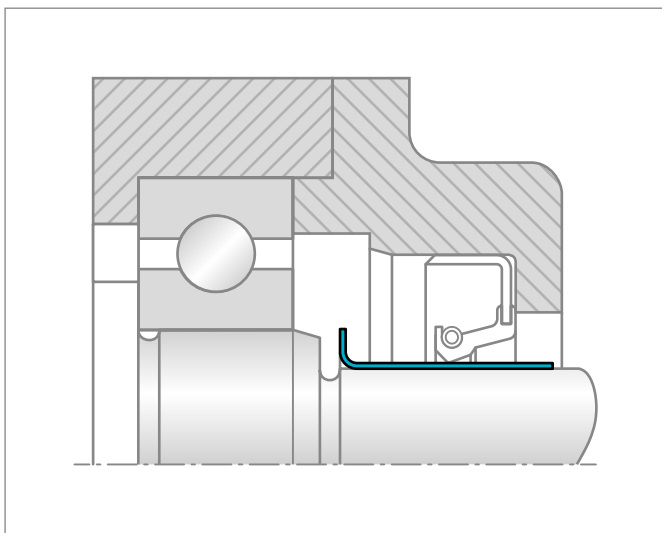
Figure 66: Running surface with shaft repair kit
