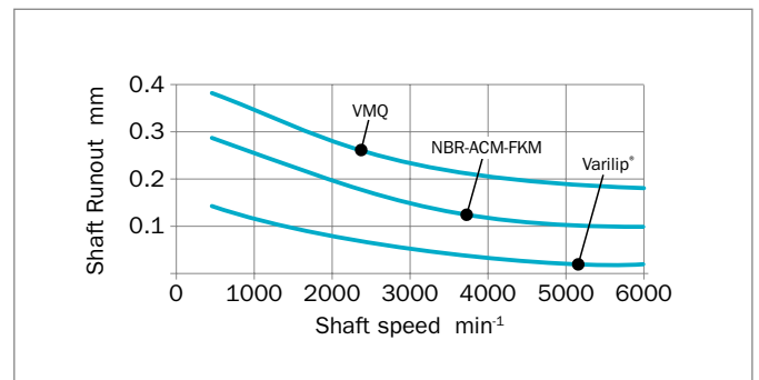
Figure 103: Dynamic eccentricity capability
