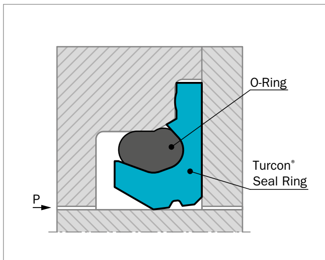
Figure 143: Turcon® Roto VL Seal® F
