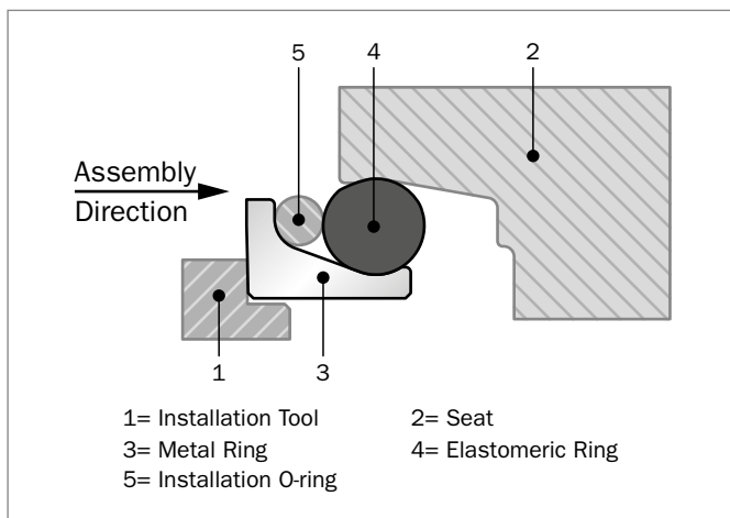
Figure 183: O-Ring as installation aid
