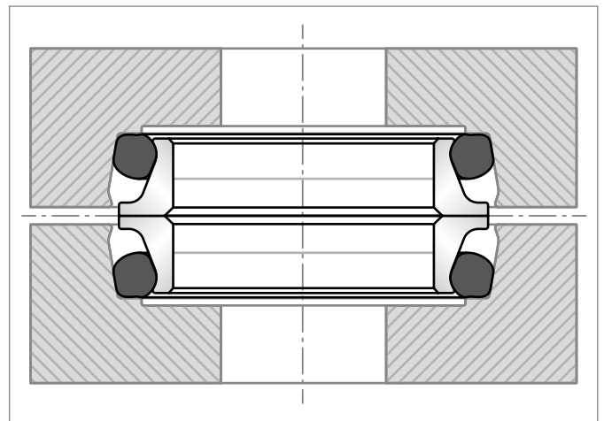
Figure 182: Both halves of the Mechanical Face Seal group have O-Rings slipped against the seat and on the seat bottom.
