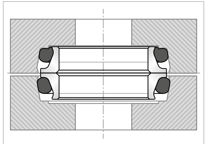
Figure 181: Upper half of the Mechanical Face Seal group has O-Ring slipped against the seat and on the seat bottom.
