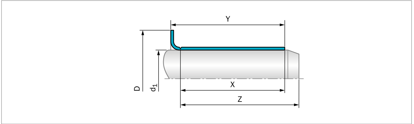
Figure 68: Installation Drawing
