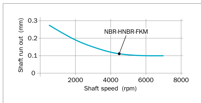
Figure 56: Permissible run out of the shaft
