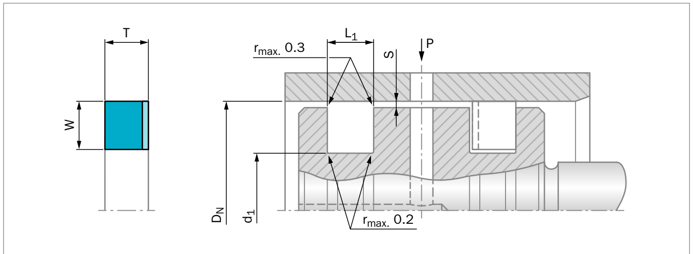
Figure 172: Installation Drawing
