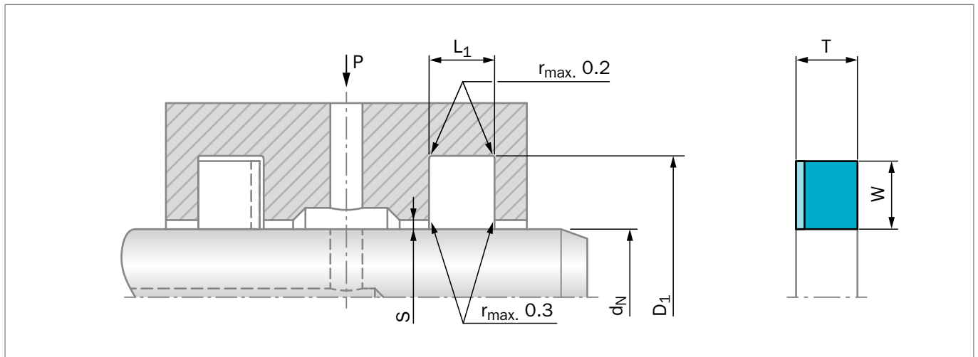
Figure 171: Installation Drawing
