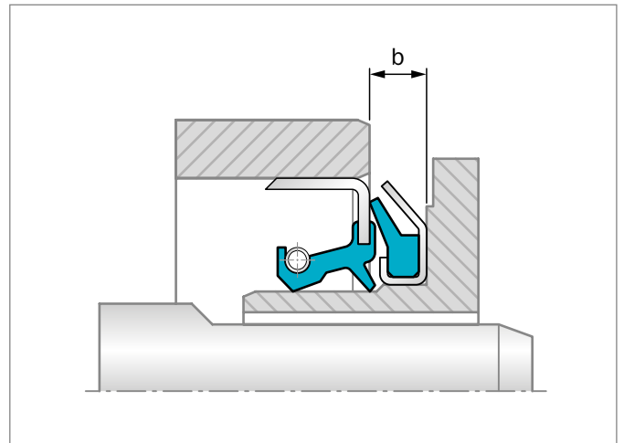
Figure 34: GAMMA seal fitted on the shaft boss
