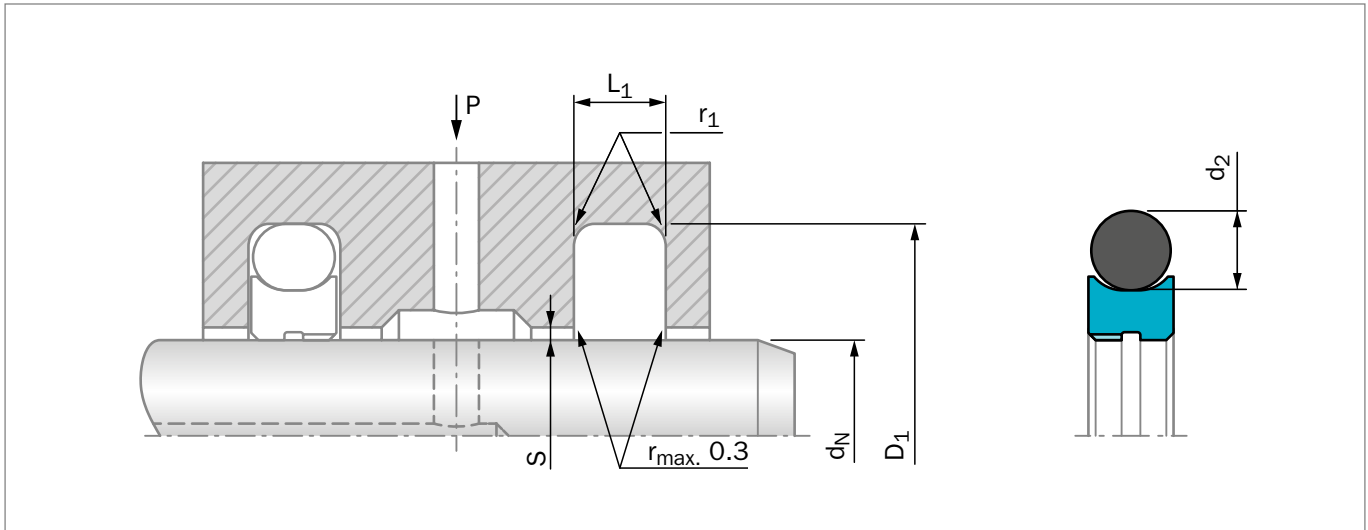
Figure 125: Installation Drawing
