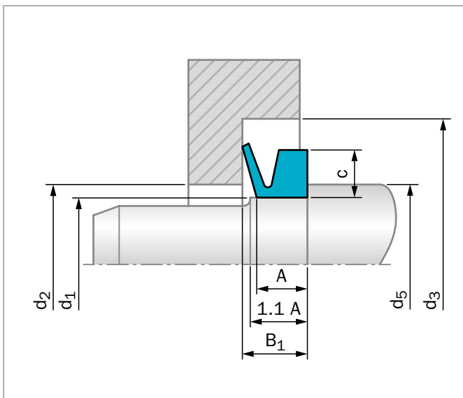
Figure 73: Axial support
