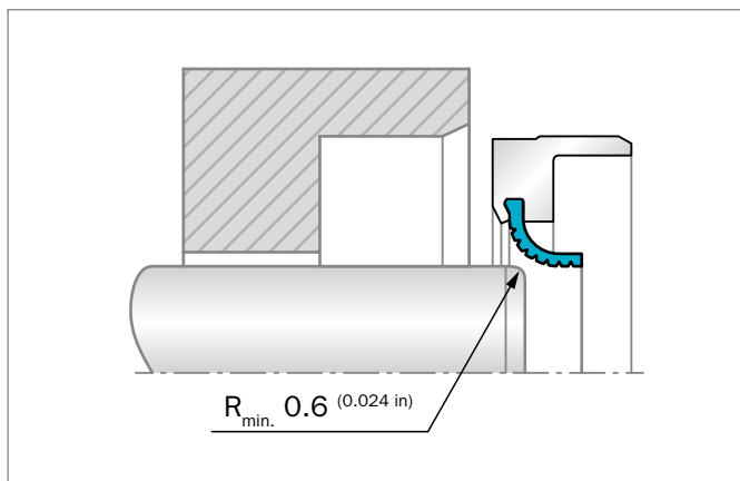
Figure 108: Installation of the sealing lip with the back to the shaft for pressurized application
