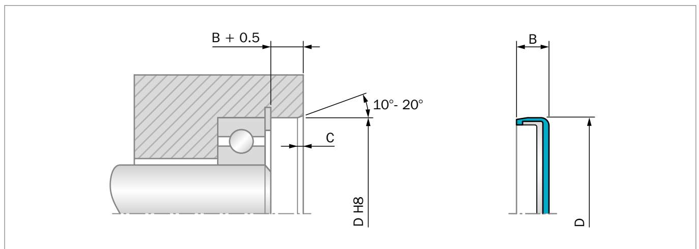
Figure 63: Installation Drawing
