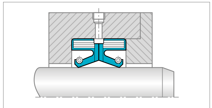
Figure 38: Type TRL mounted back to back
