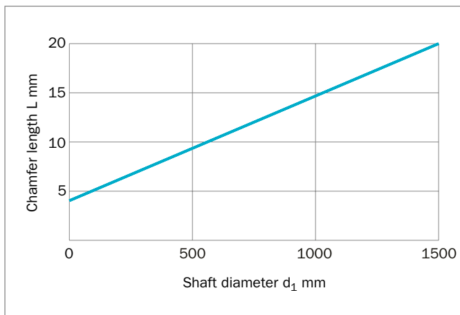
Figure 41: Chamfer length as a function of the shaft diameter
