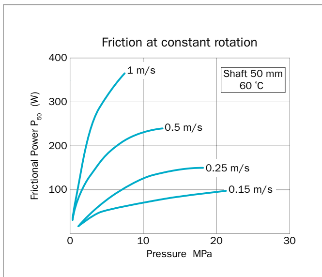
Figure 139 Frictional power for Turcon® Roto Variseal®
