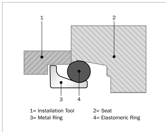
Figure 176: Installation Tool for DO Type
