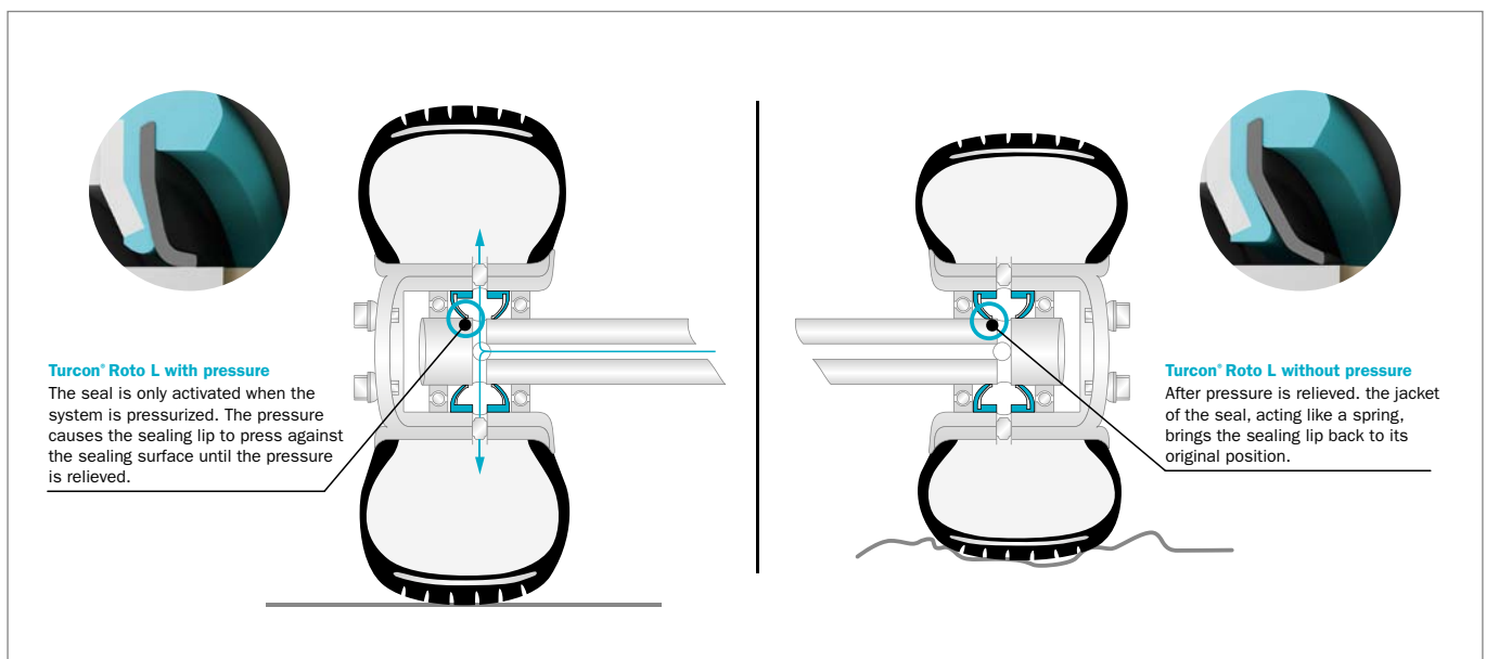
Figure 92: Functional Principle Turcon® Roto L
