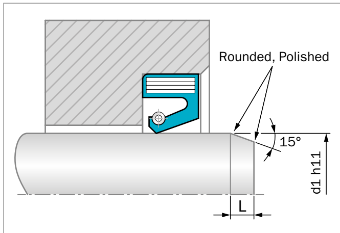
Figure 40: Installation of the oil seal
