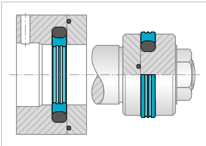
Figure 152: Installation of Roto Glyd Ring® in split groove
