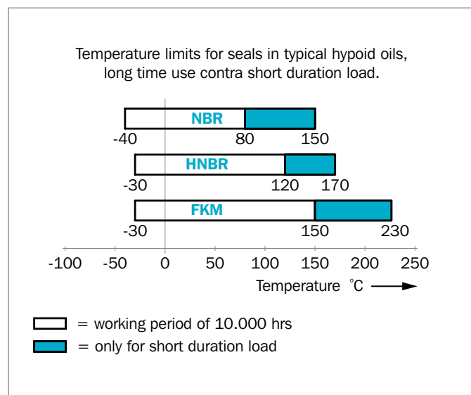
Figure 53: Temperature recommendations in typical hypoid oils
