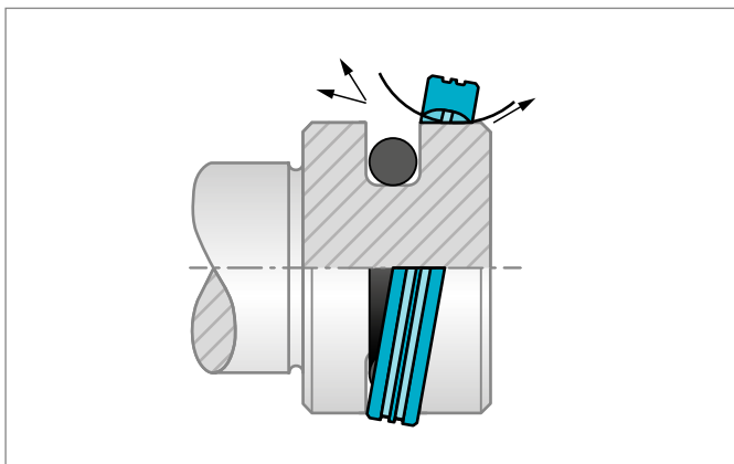
Figure 165: Schematic installation of the Turcon® seal ring
