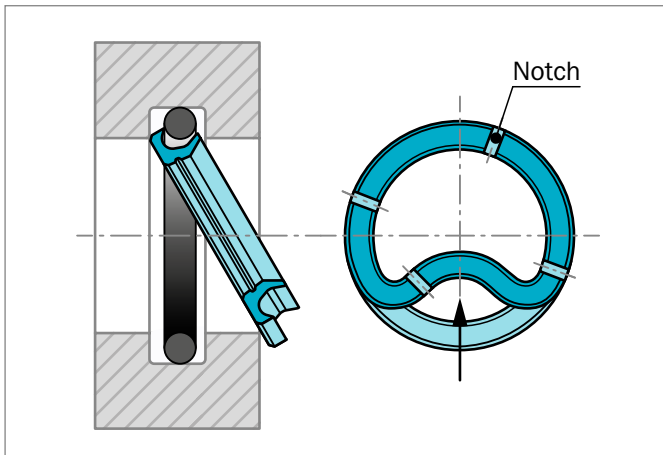
Figure 160: Installation of shaft Turcon® Roto VL Seal® in closed groove
