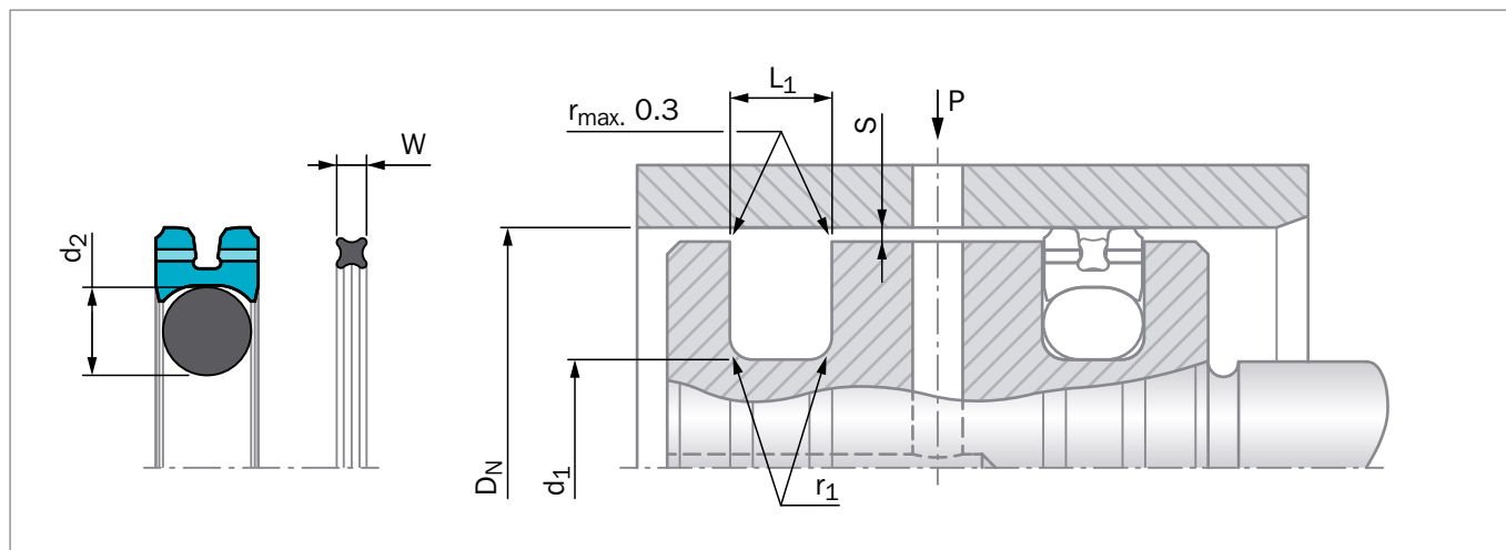
Figure 132 Installation Drawing
