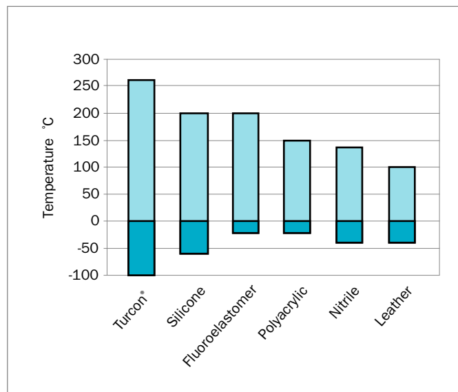
Figure 101: Maximum and minimum temperatures for different materials
