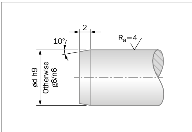
Figure 85: Tolerance of the shaft, surface roughness and chamfer of the shaft
