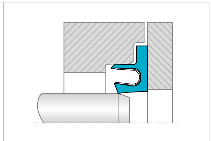
Figure 141 Turcon® Roto Variseal®
