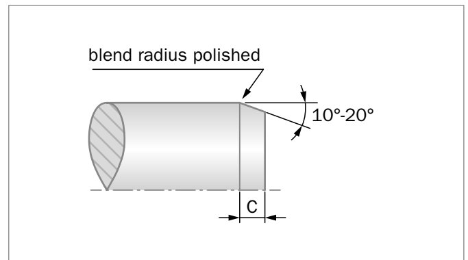
Figure 166: Lead-in chamfer on shaft
