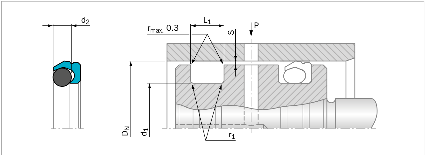
Figure 151: Installation Drawing
