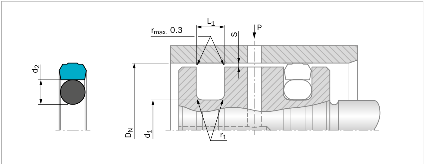
Figure 137 Installation Drawing
