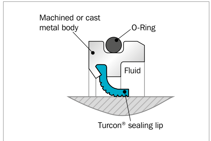
Figure 97: O-Ring design
