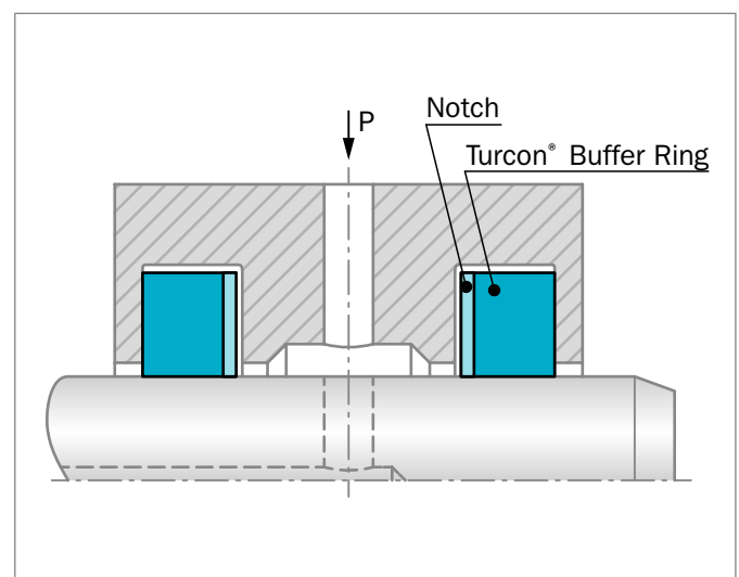
Figure 169: Right installation of Turcon® Buffer Ring
