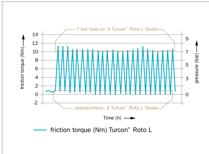
Figure 93: Dry air torque tes
