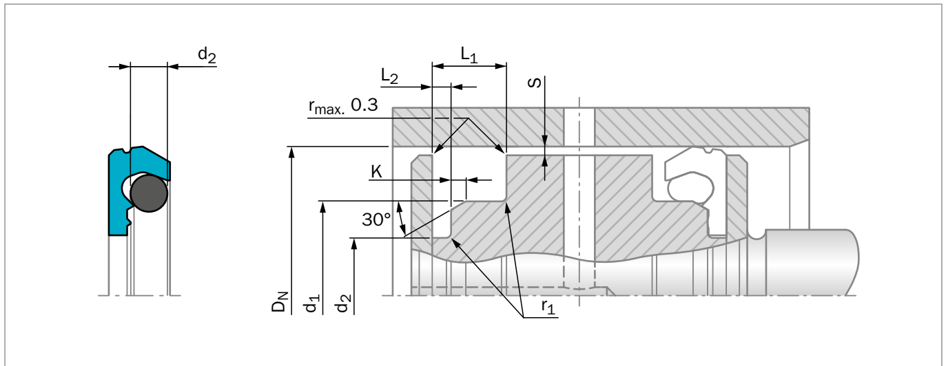
Figure 146: Installation Drawing
