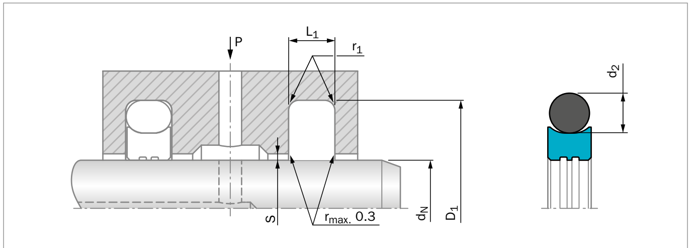
Figure 120: Installation Drawing
