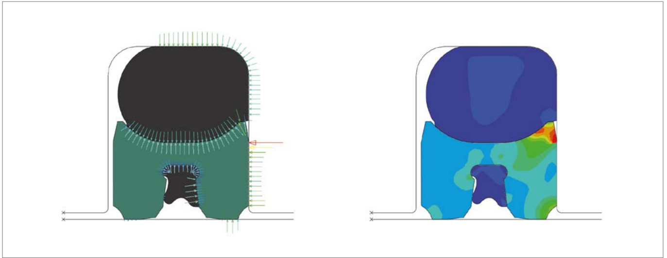
Figure 128 Turcon® Roto Glyd Ring® V - Finite Element Analysis (FEA).
