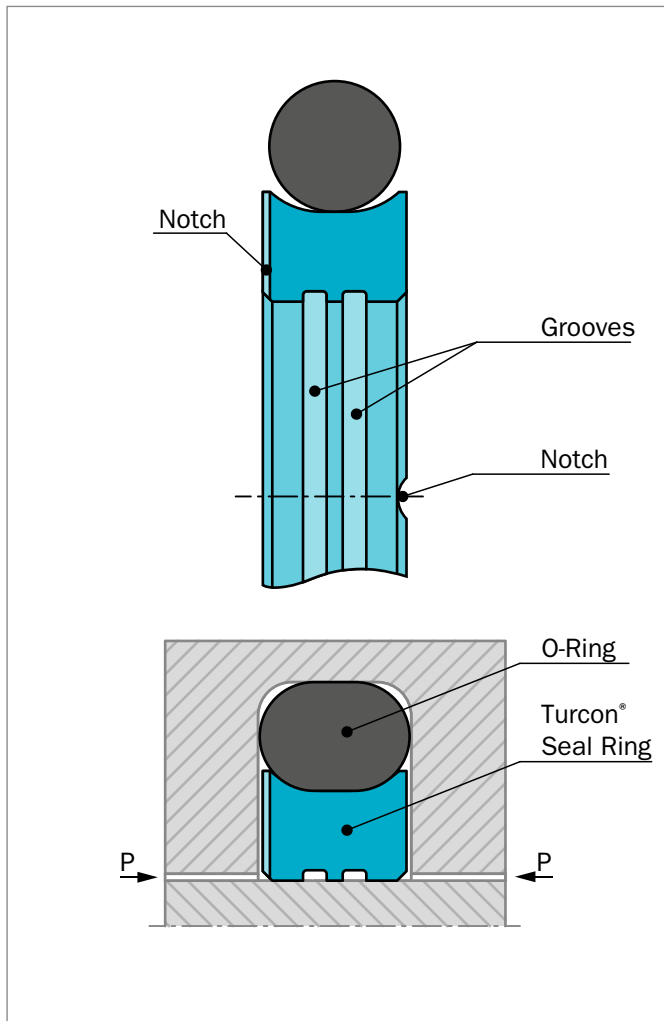
Figure 117: Turcon® Roto Glyd Ring®
