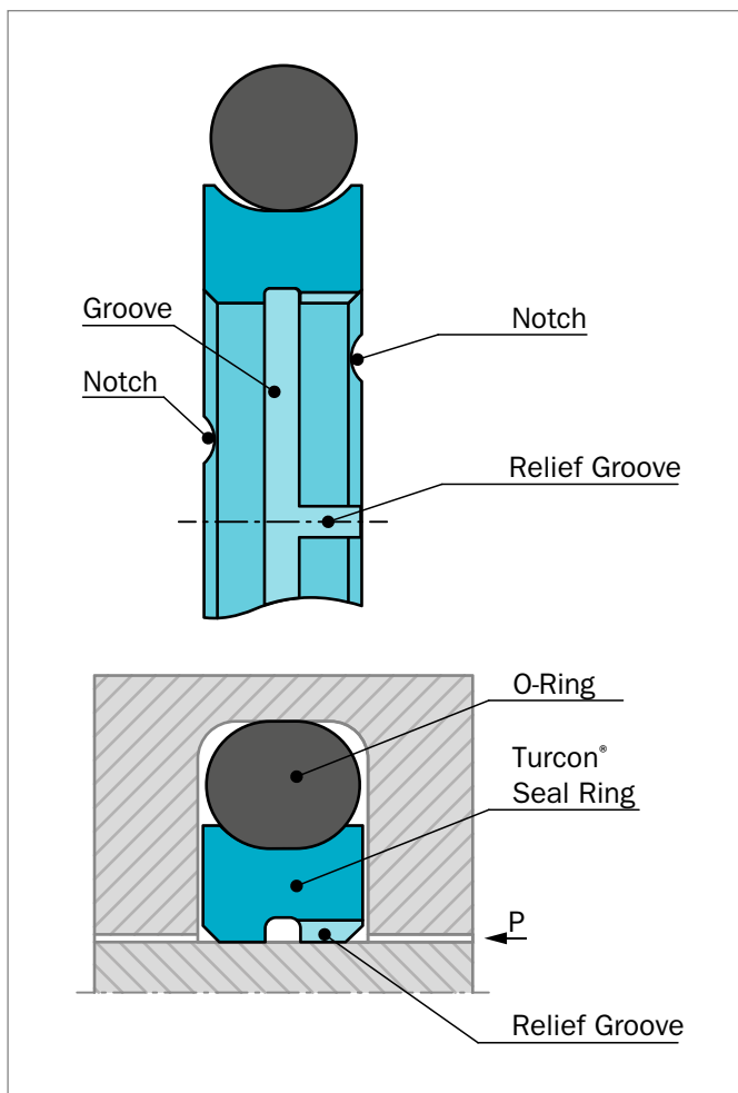
Figure 122: Turcon® Roto Glyd Ring® K with pressure relief.
