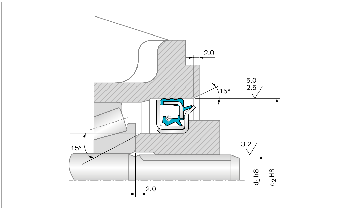
Figure 55: System 5000 in pinion application
