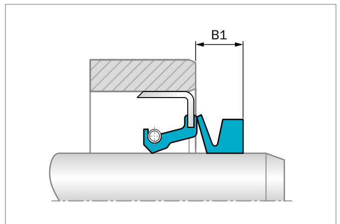
Figure 35: V-Ring fitted on the shaft end
