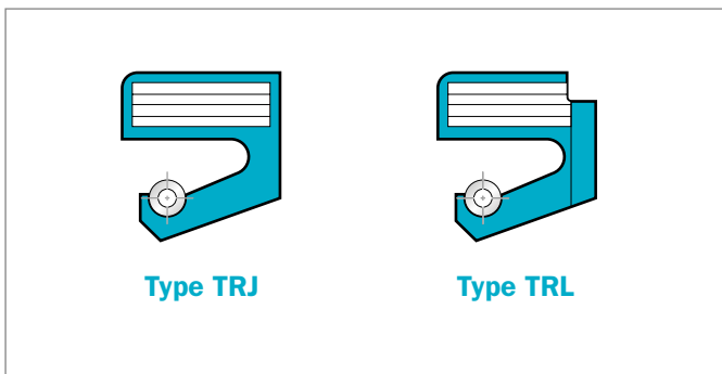
Figure 36: Fiber reinforced design for large diameters
