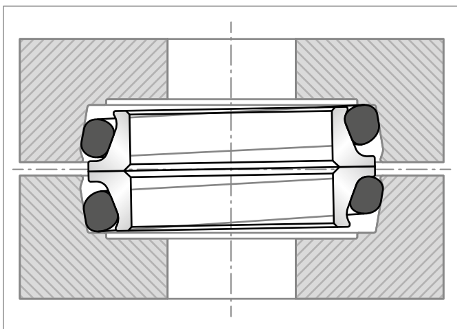
Figure 180: O-Rings slipped against seats and Mechanical Face Seal group is tilted.
