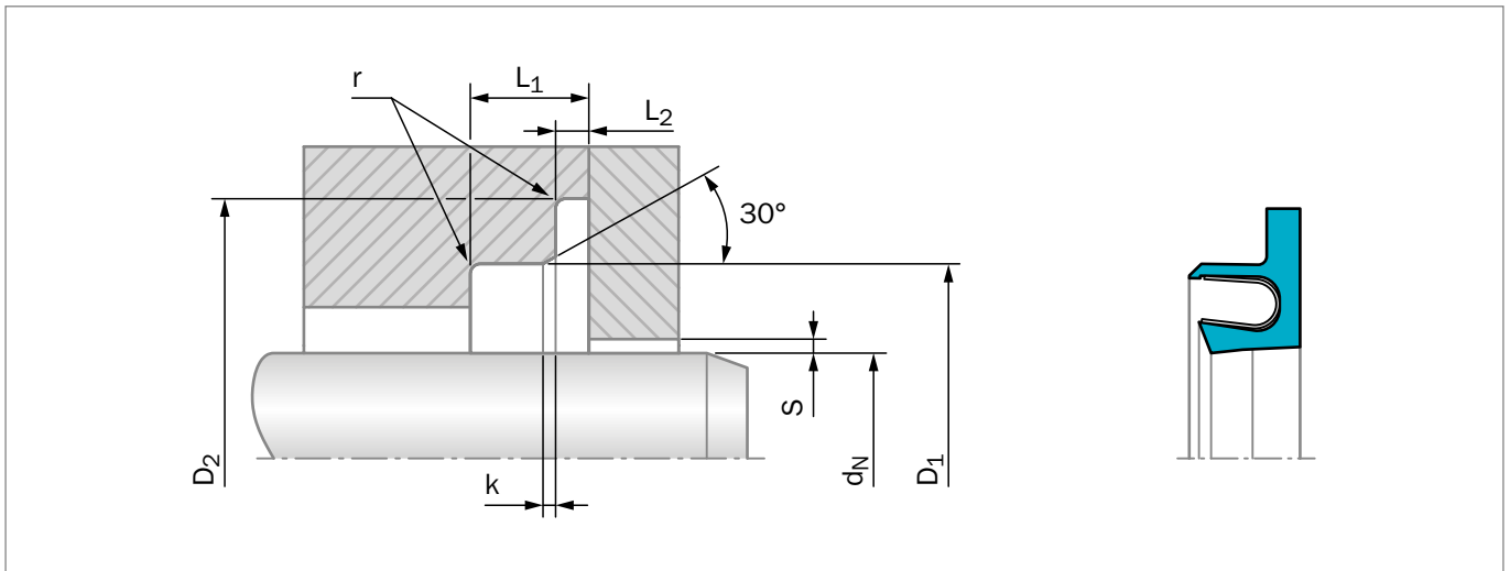
Figure 142 Installation Drawing
