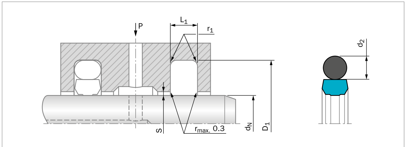
Figure 136 Installation Drawing
