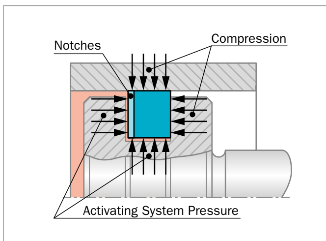
Figure 168: Pressure activation of Turcon® Buffer Ring
