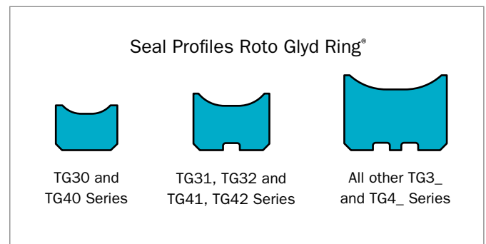
Figure 118: Crosssection profiles depending on Series No.
