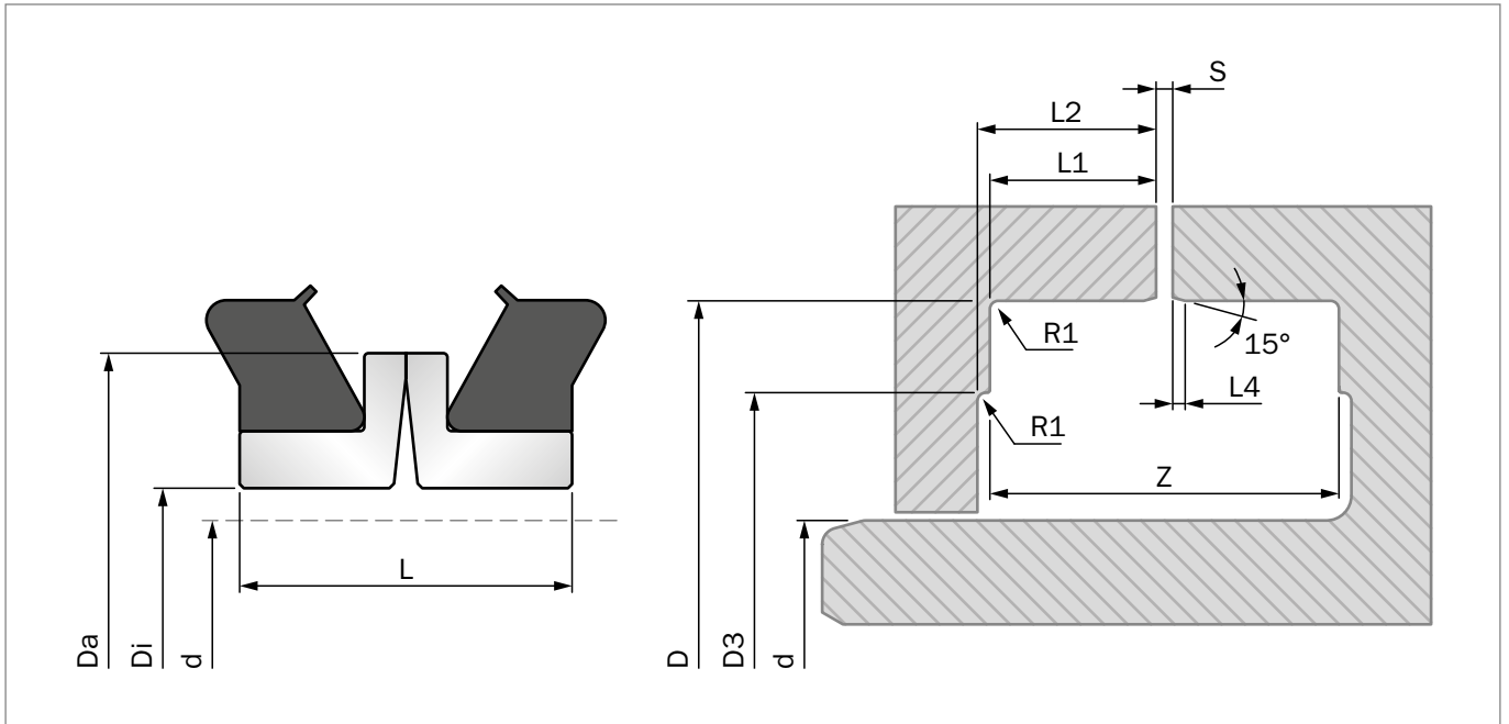
Figure 186: Installation Drawing
