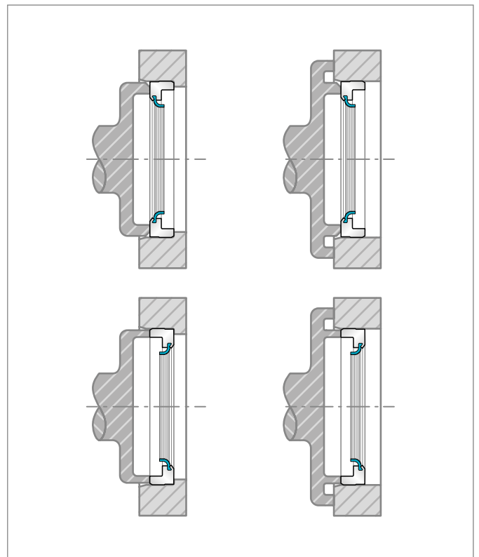
Figure 112: Assembly tooling types for press fit into a housing
