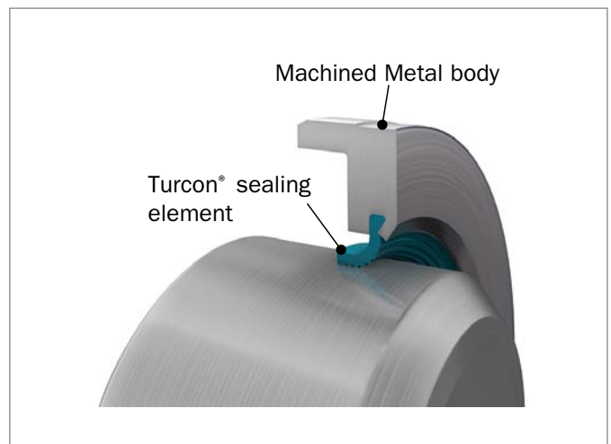
Figure 95: Turcon® Varilip® PDR seal
