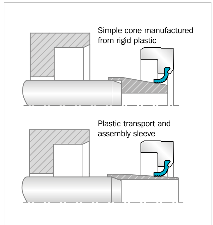
Figure 111: Assembly tooling types for installation on shafts
