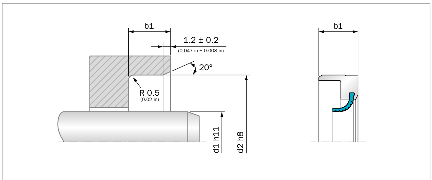
Figure 113: Installation drawing for pressure up to 0.5 MPa (73 psi)
