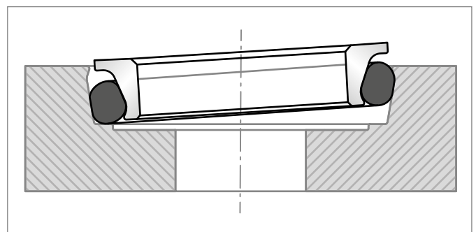
Figure 178: O-Ring slipped against the seat.
