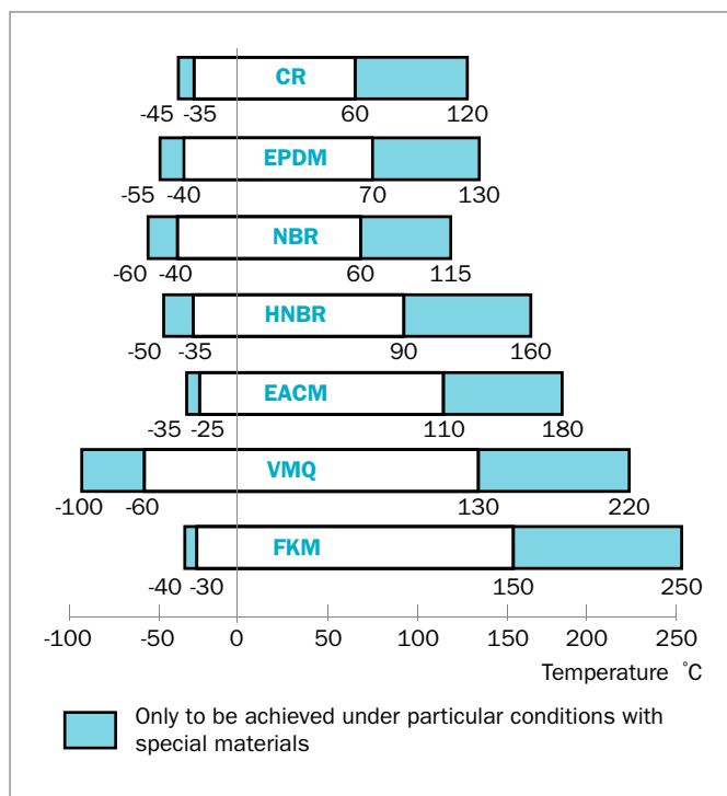
Figure 72: Temperature recommendations for V-Rings
