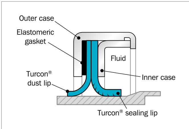
Figure 96: Clamped design
