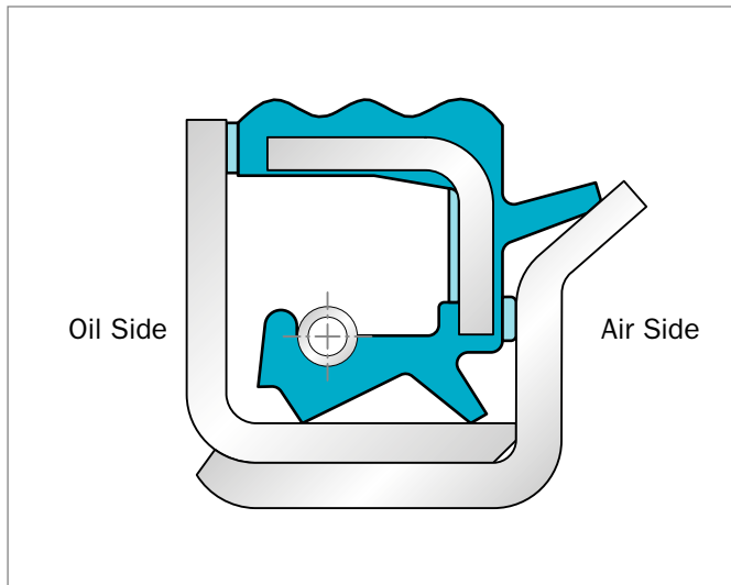
Figure 50: System 5000
