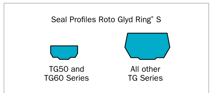
Figure 135 Cross-section profiles depending on Series No.
