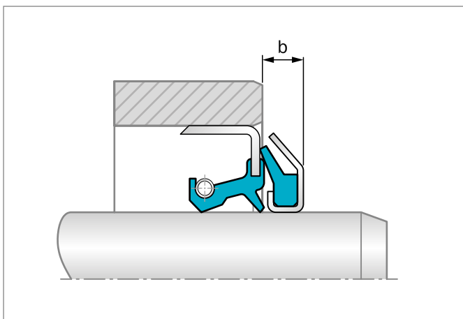
Figure 33: GAMMA seal fitted on the shaft end
