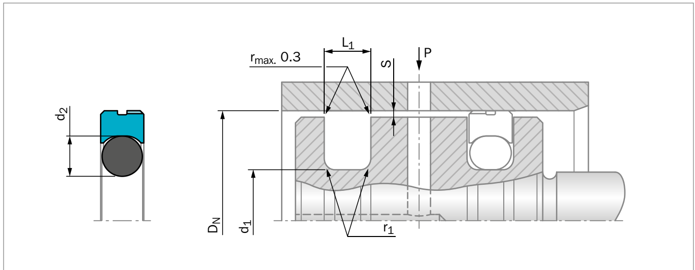
Figure 126: Installation Drawing
