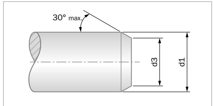
Figure 109: Shaft lead-in chamfer
