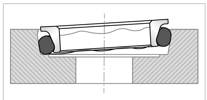
Figure 179: O-Ring slipped against the seat and waved against the metal ring.
