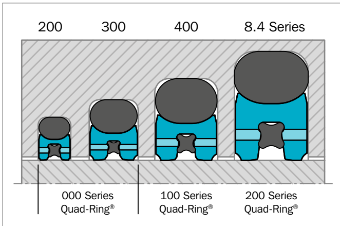
Figure 129 Cross-section profiles of available standard seal series for shaft and bore sealing dependent on Series No.
