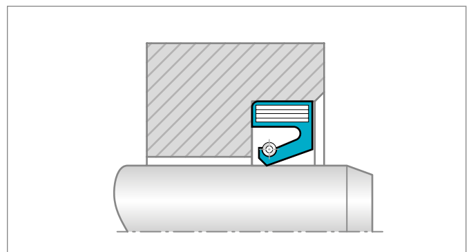
Figure 39: Type TRJ/F mounted without axial retaining plate
