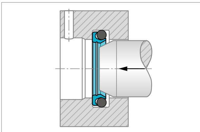
Figure 161: Direction of calibration of installed Roto VL Seal®
