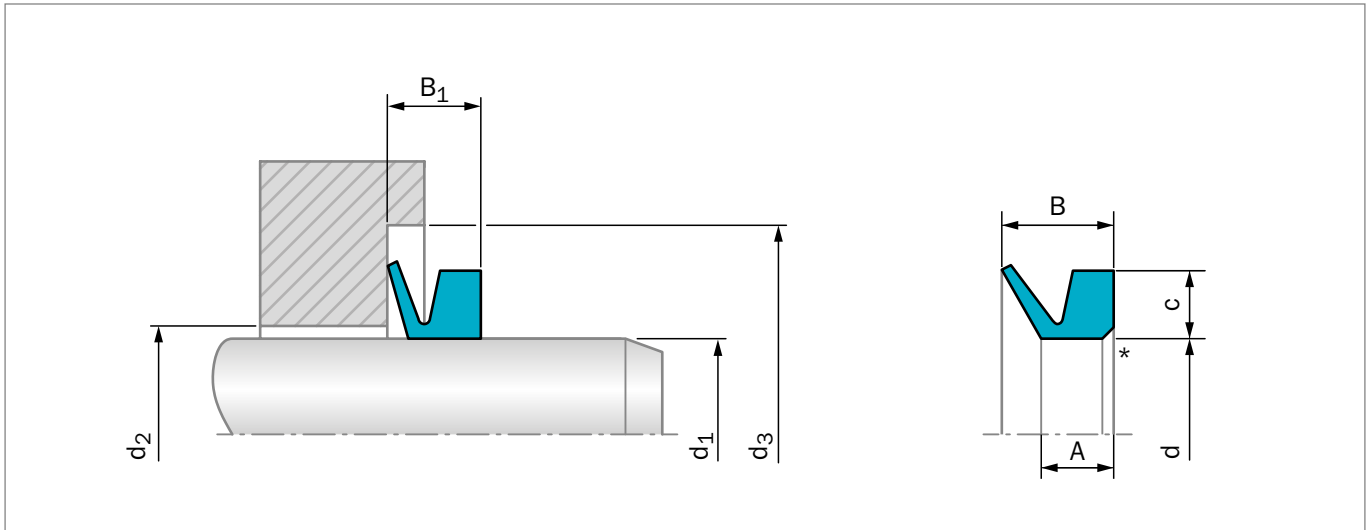
Figure 76: Installation Drawing
