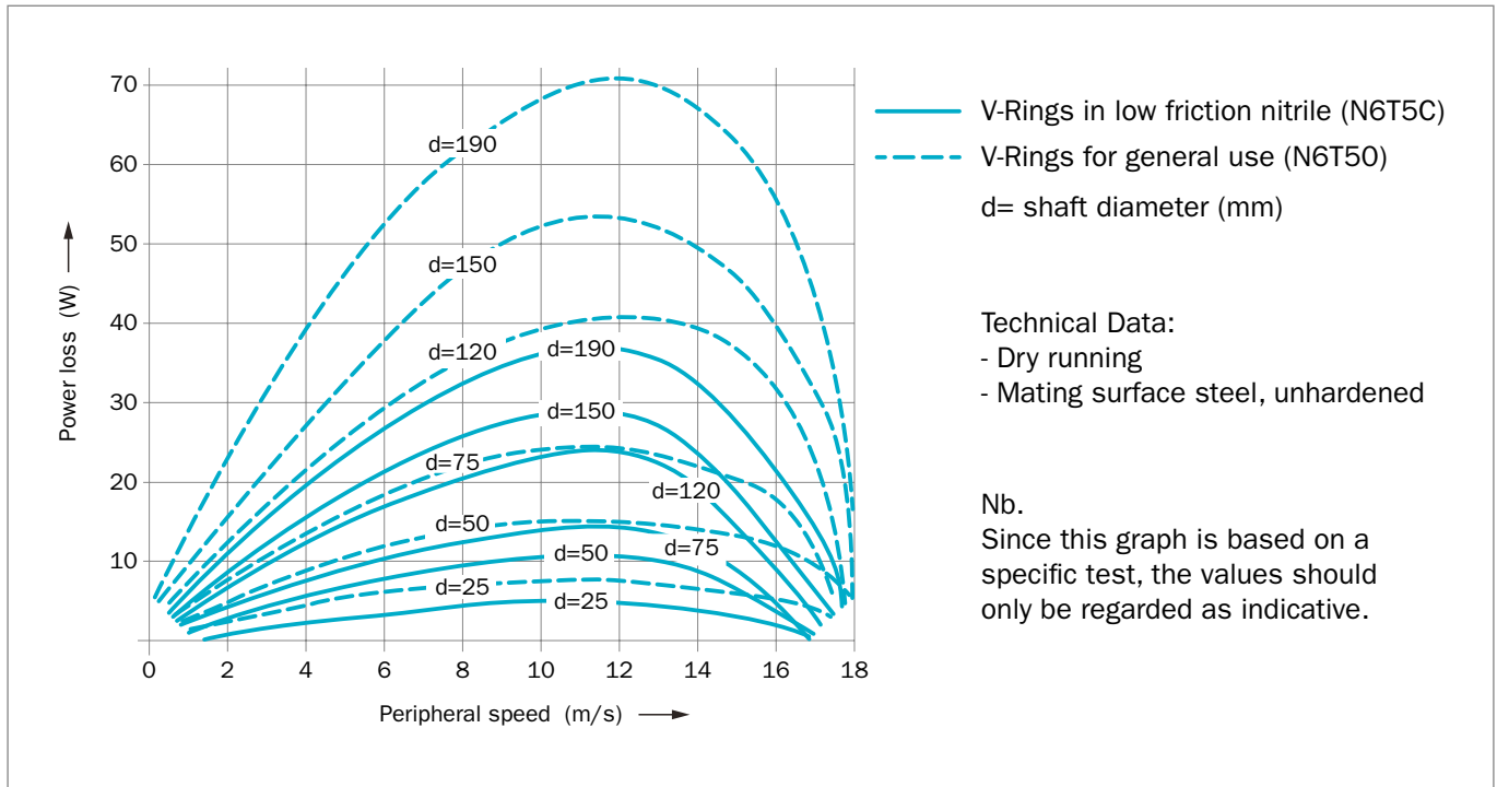
Figure 71: Power loss as a function of peripheral speed for various sizes
