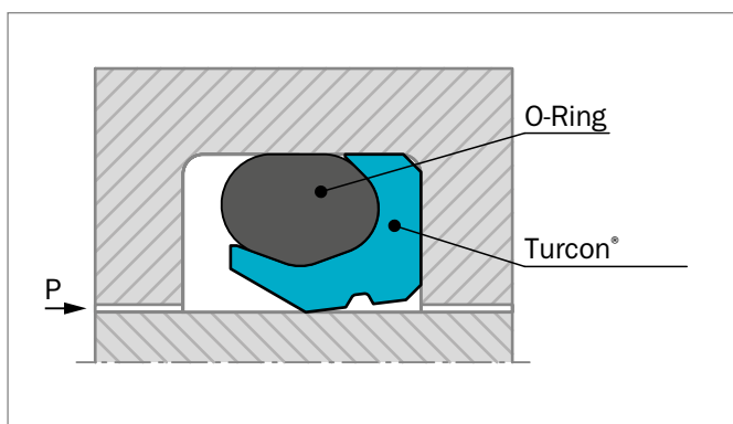
Figure 147: Turcon® Roto VL Seal®
