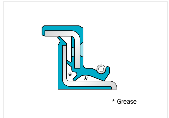
Figure 61: "Hygienic design" APJ for food applications
