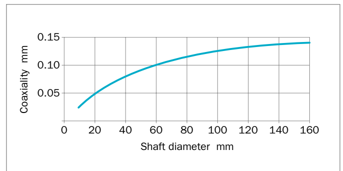
Figure 104: Coaxial tolerance capability
