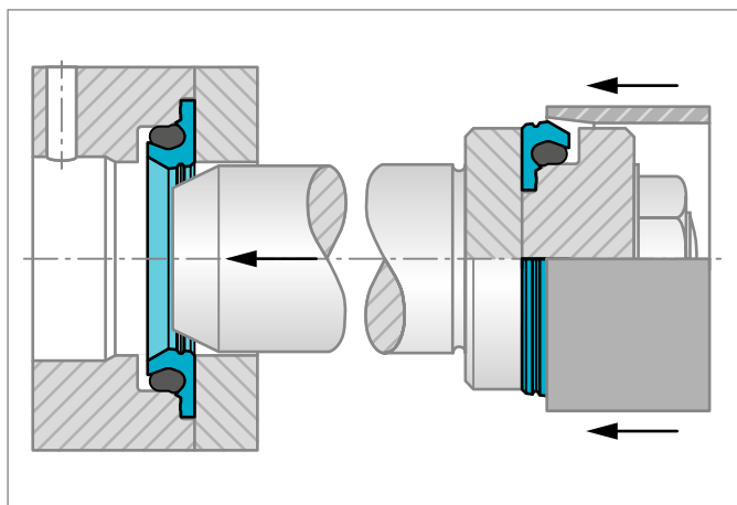
Figure 156: Installation of rod Turcon® Roto Variseal® and Roto VL Seal® F in split groove
