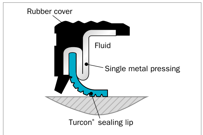
Figure 98: Single shell design
