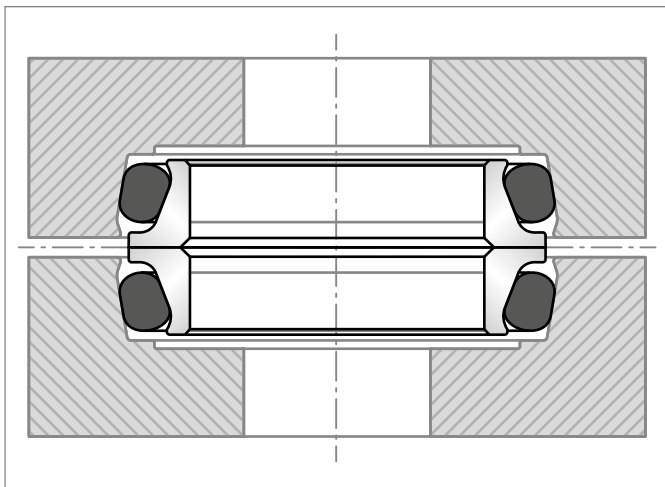
Figure 181: Upper half of the Mechanical Face Seal group has O-Ring slipped against the seat and on the seat bottom.
