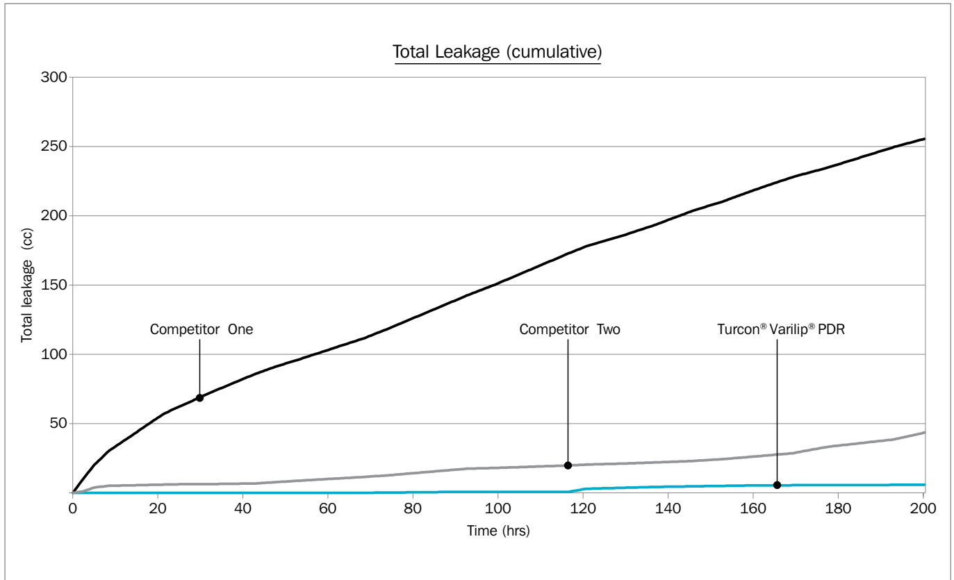
Figure 106: Total leakage (cumulative) monitored over 200 hour tests (average results)
