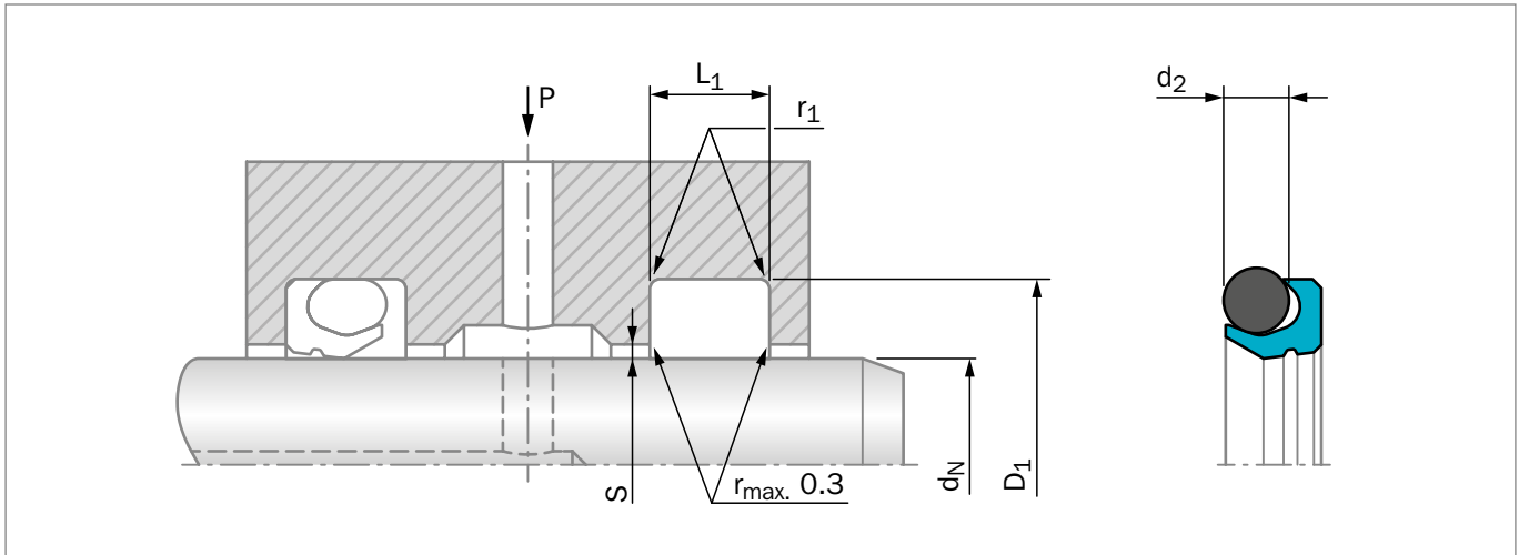
Figure 150: Installation Drawing
