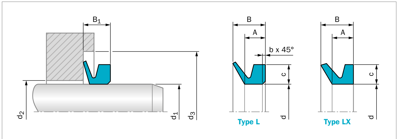
Figure 78: Installation Drawing
