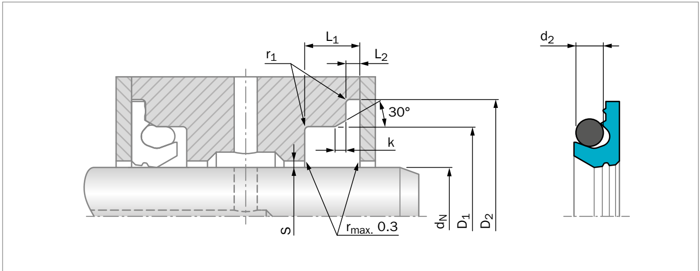
Figure 145: Installation Drawing
