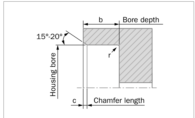
Figure 107: Housing design schematic
