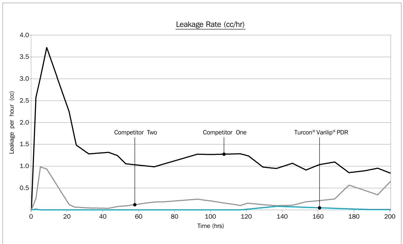
Figure 105: Leakage rate per hour monitored over 200 hour tests (average results)
