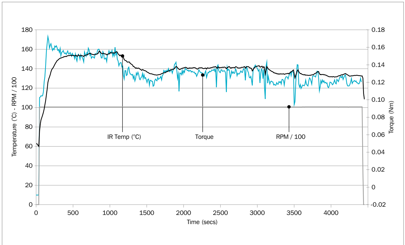
Figure 102: Running torque for Turcon® Varilip® PDR seal
