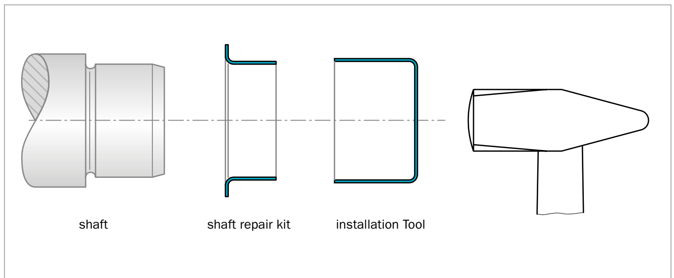
Figure 67: Installation sequence
