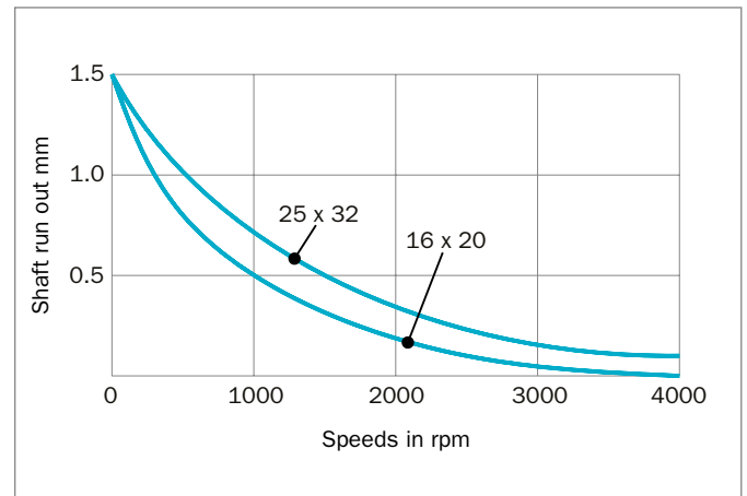
Figure 42: Shaft run out
