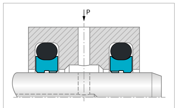
Figure 123: Right installation of Roto Glyd Ring® K
