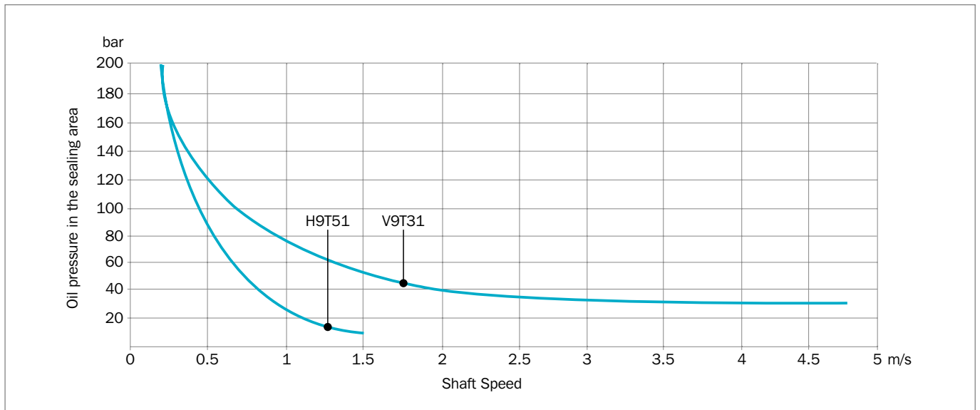
Figure 25: HP20 Rated Working Conditions
