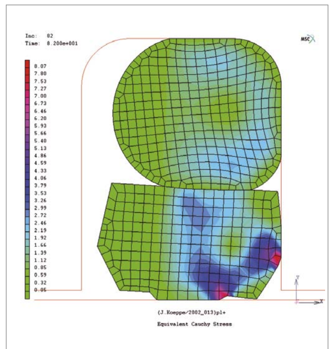
Figure 134 Zurcon® Roto Glyd Ring® S - Finite Element Analysis (FEA)
