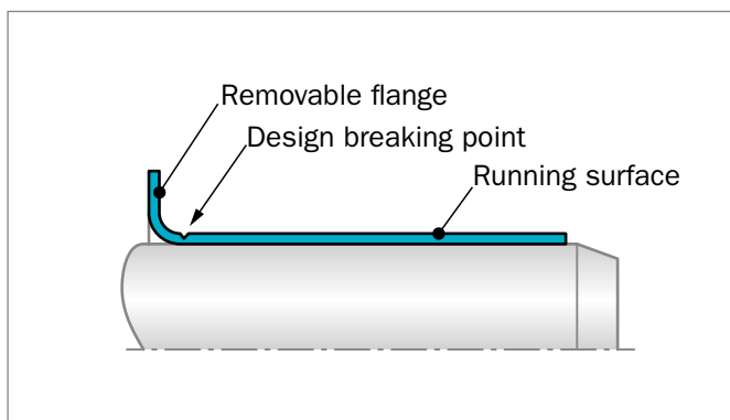
Figure 65: Design of the shaft repair kit
