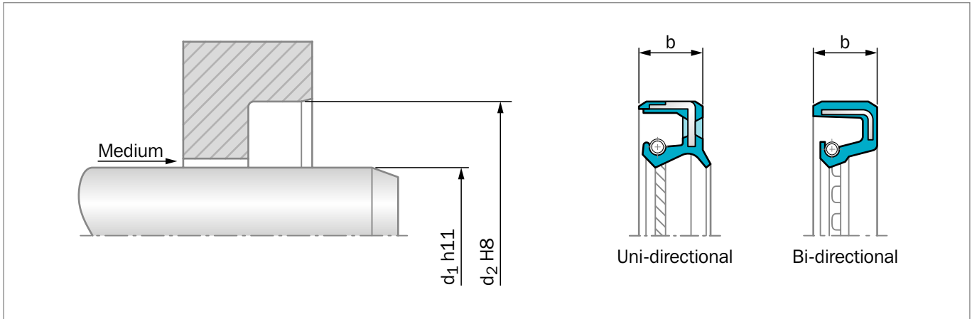
Figure 31: Installation Drawing
