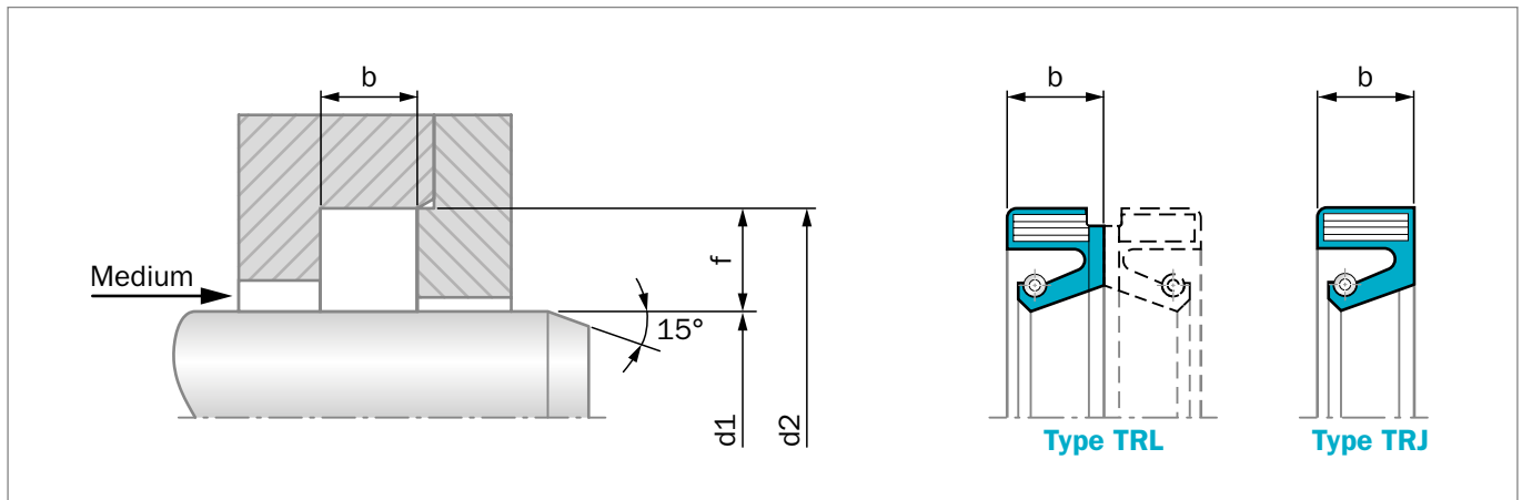
Figure 45: Installation Drawing
