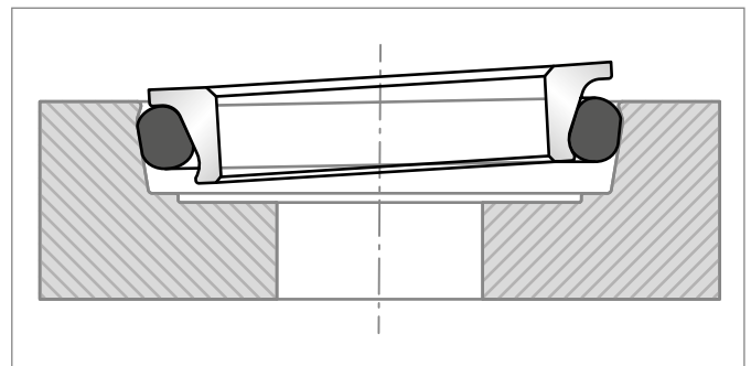
Figure 177: Metal ring slipped against the O-Ring
