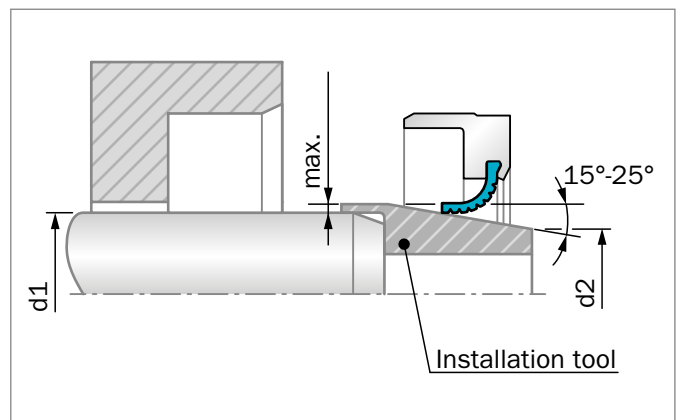
Figure 110: Fitting the sealing lip using an installation tool
