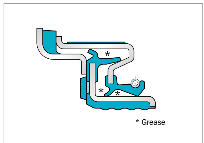
Figure 62: APJ for heavy polluted applications and axial play of the shaft
