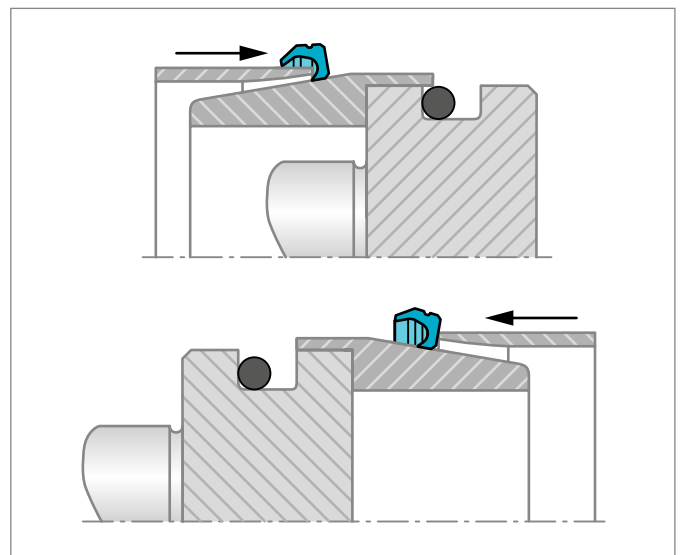
Figure 163: Installation of bore Turcon® Roto VL Seal® in closed groove using an expanding pusher over an installation cone
