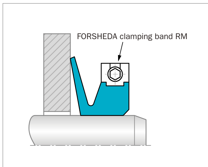
Figure 75: Clamping Band RM
