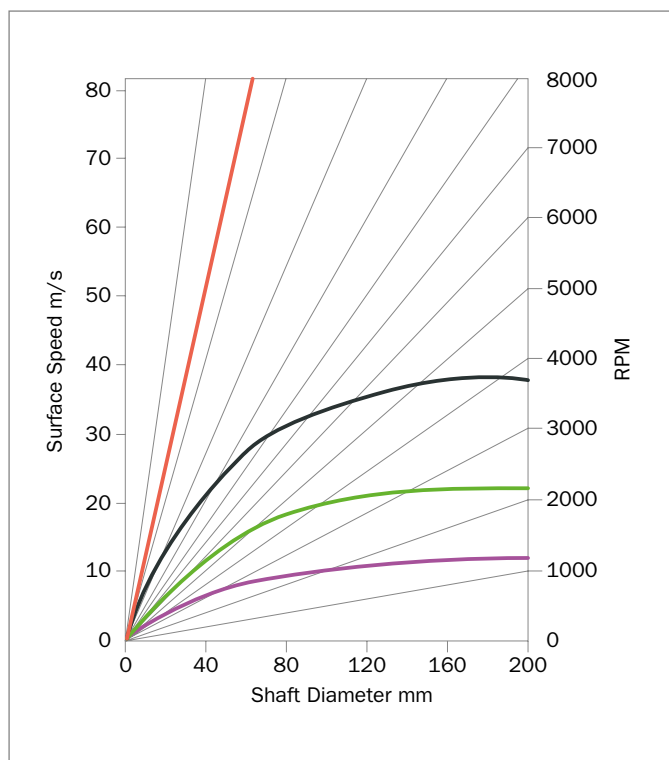
Figure 100: Surface speed as a function of shaft diameter and RPM
