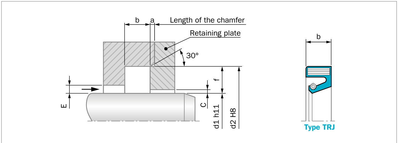
Figure 43: Installation Drawing
