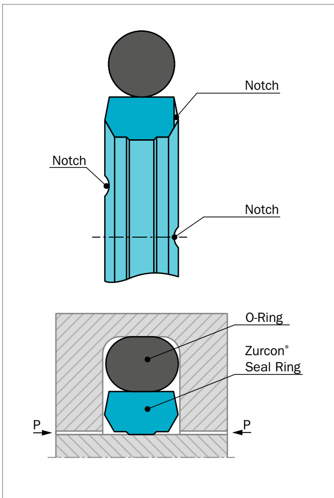
Figure 133 Zurcon® Roto Glyd Ring® S
