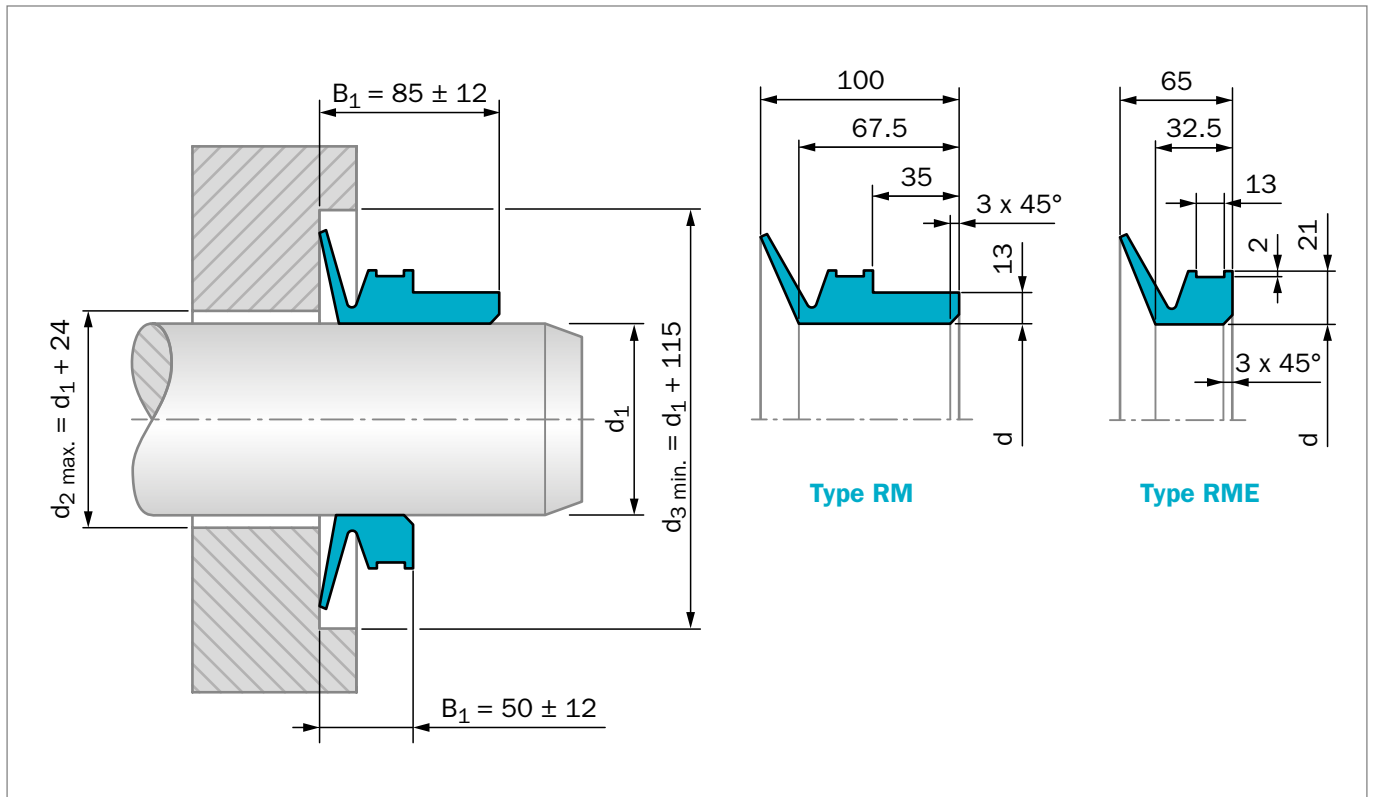
Figure 79: Installation Drawing
