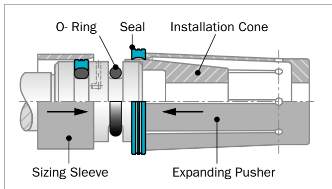
Figure 162: Expanding the Turcon® Roto Glyd Ring® etc. over the Installation Cone using an Expanding Pusher
