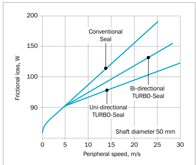
Figure 32: Friction loss
