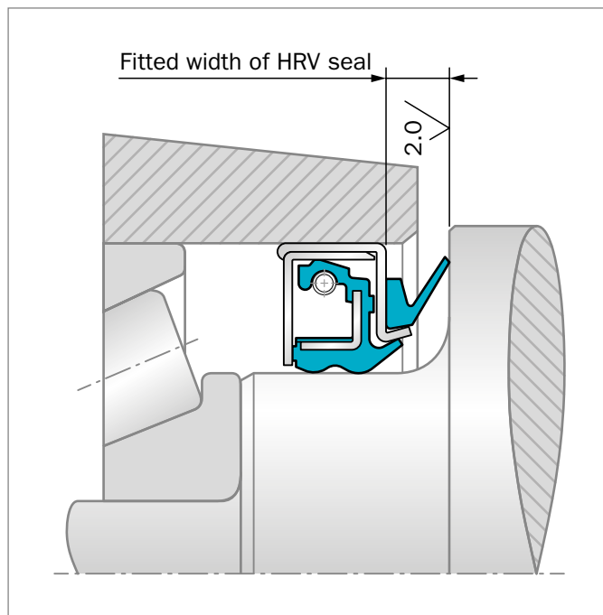
Figure 58: System 500 with HRV seal
