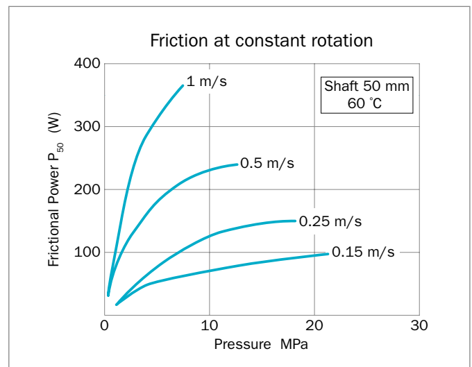
Figure 124: Frictional power for Turcon® Roto Glyd Ring® K
