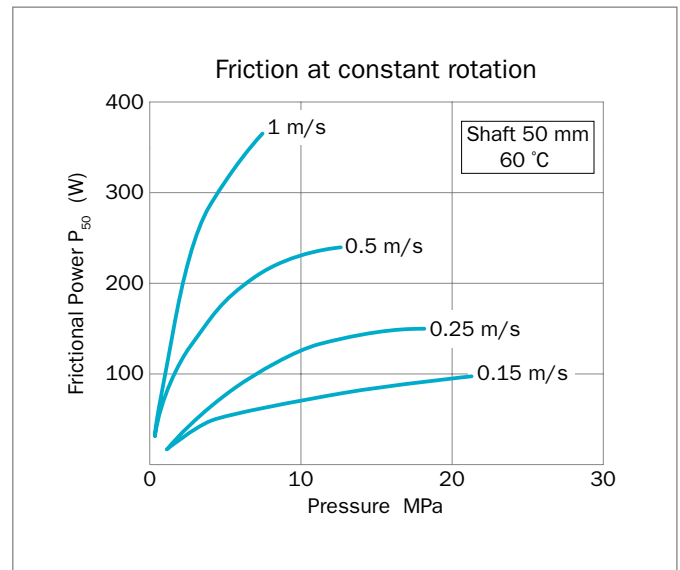
Figure 119: Frictional power for Turcon® Roto Glyd Ring®
