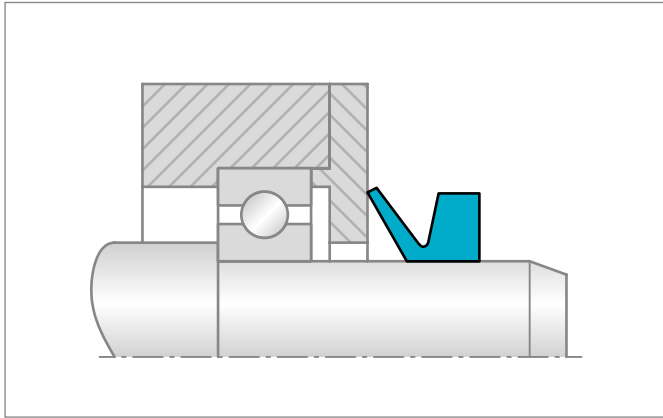
Figure 70: Method of operation of the V-Ring
